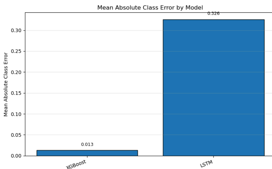
Figure 5: Mean Absolute Class Error by XGBoost and LSTM.
